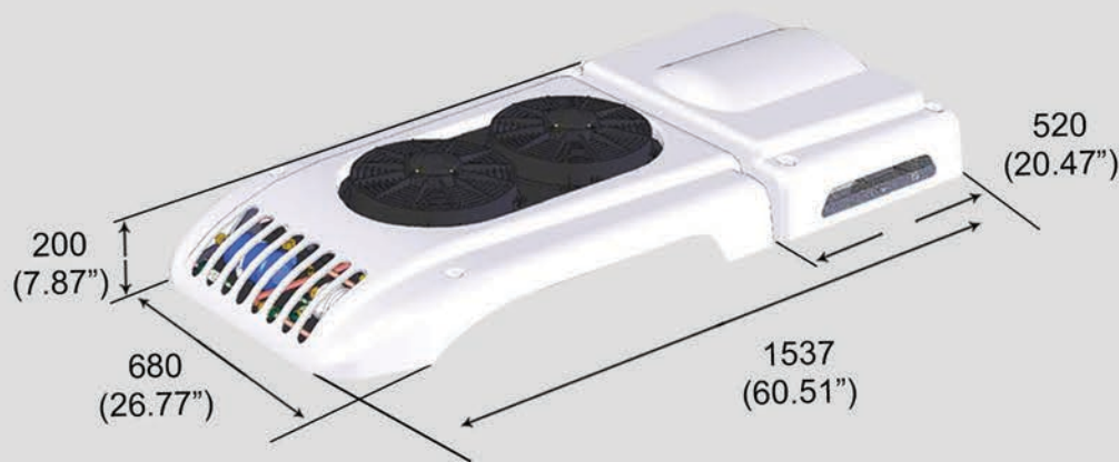
T235D Condenser
