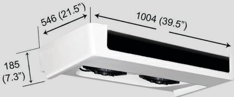
EVK300C EVAPORATOR ASSEMBLY
