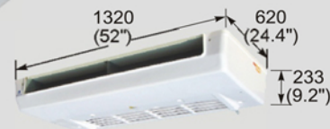
EVK500 Evaporator Assembly
